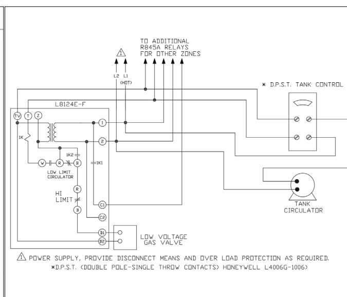
Figure 16 - Zoning with Circulators Using L8124 A, C, and DPST Control - No Relay Required
