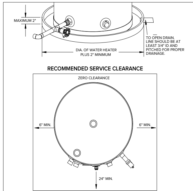
Figure 1 - Drain Pan Installation and Recommended Service Clearances
